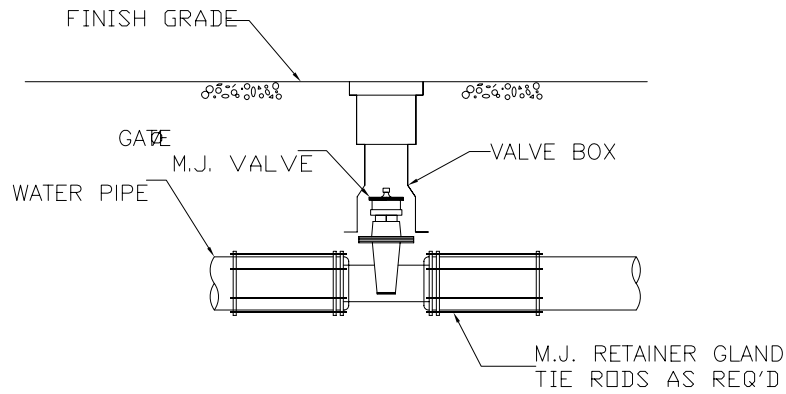
VALVE DETAIL NTS
